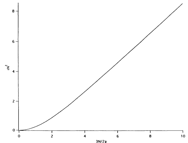
FIG. 3. Plot of elastic modulus \varepsilon N^2 as a function of x = 3N/2a for polymer chains of arbitrary stiffness a .
